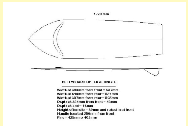
Leigh Tingle board specifications.
